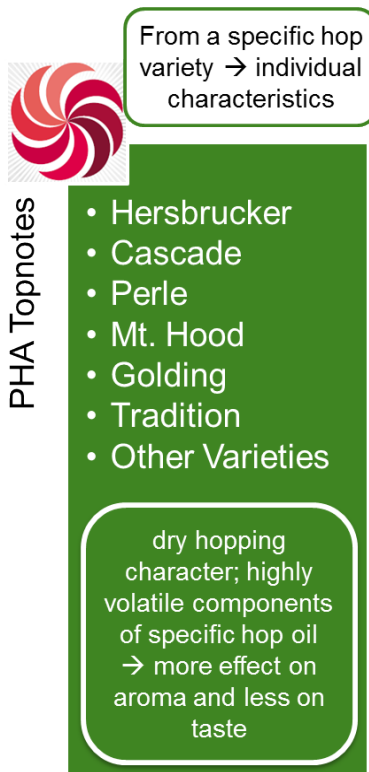
Figure 1: PHA® Topnotes
